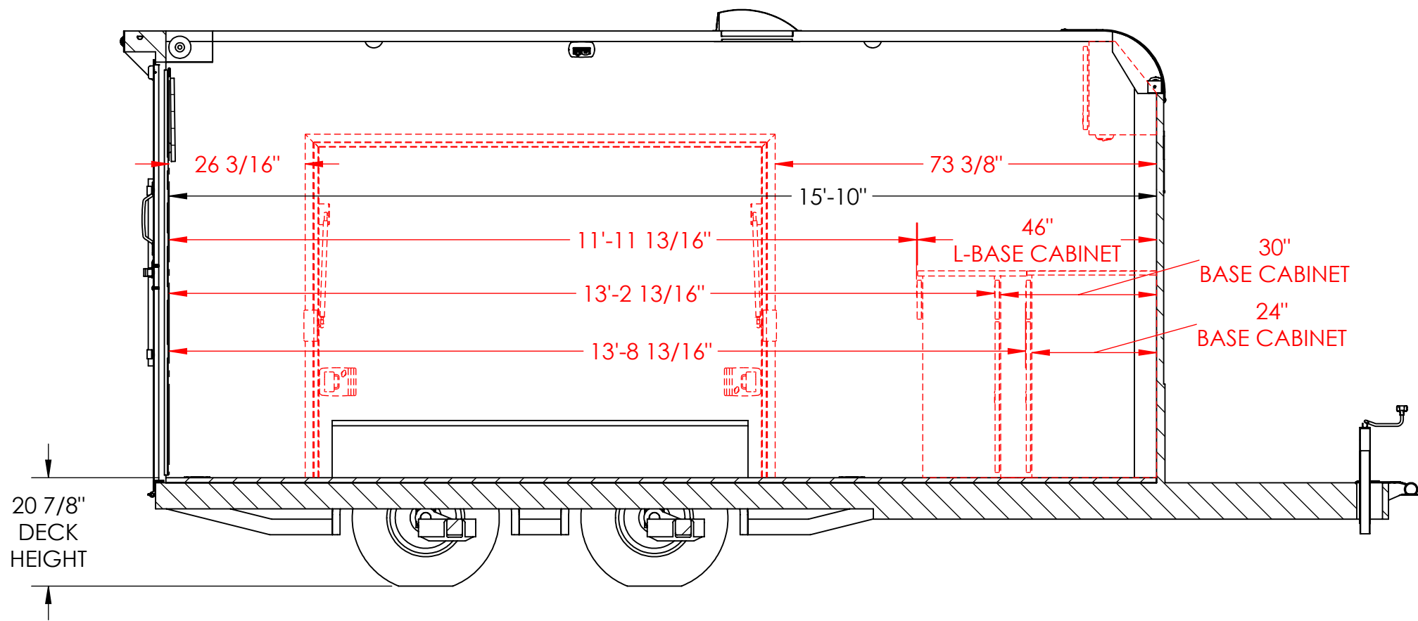
INTERIOR ROAD SIDE SECTION A-A
